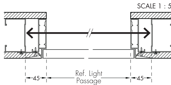
4 sides frame
